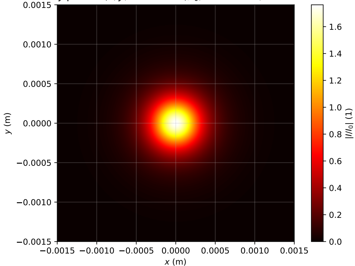
Intensity profile I(x, y, z = 1.353m)/I_0 , Pin=1.0Pcr, artificial time
